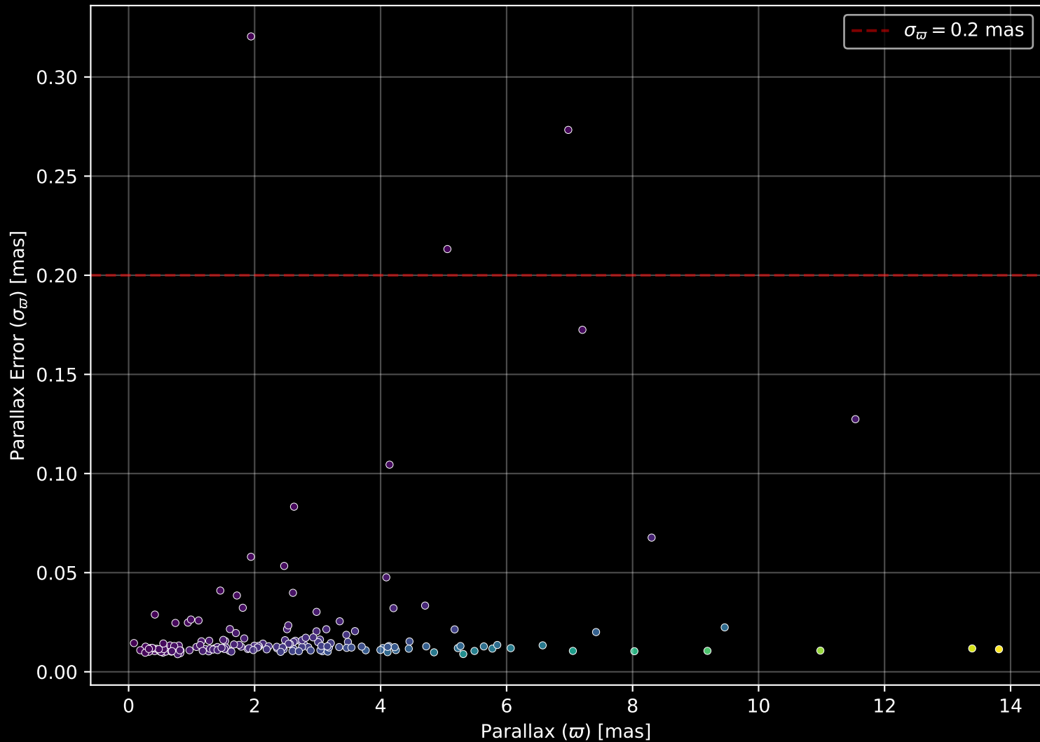
APOGEE DR17 Field: [CVZ_OB02_btx] Parallax Quality (n= 165)
