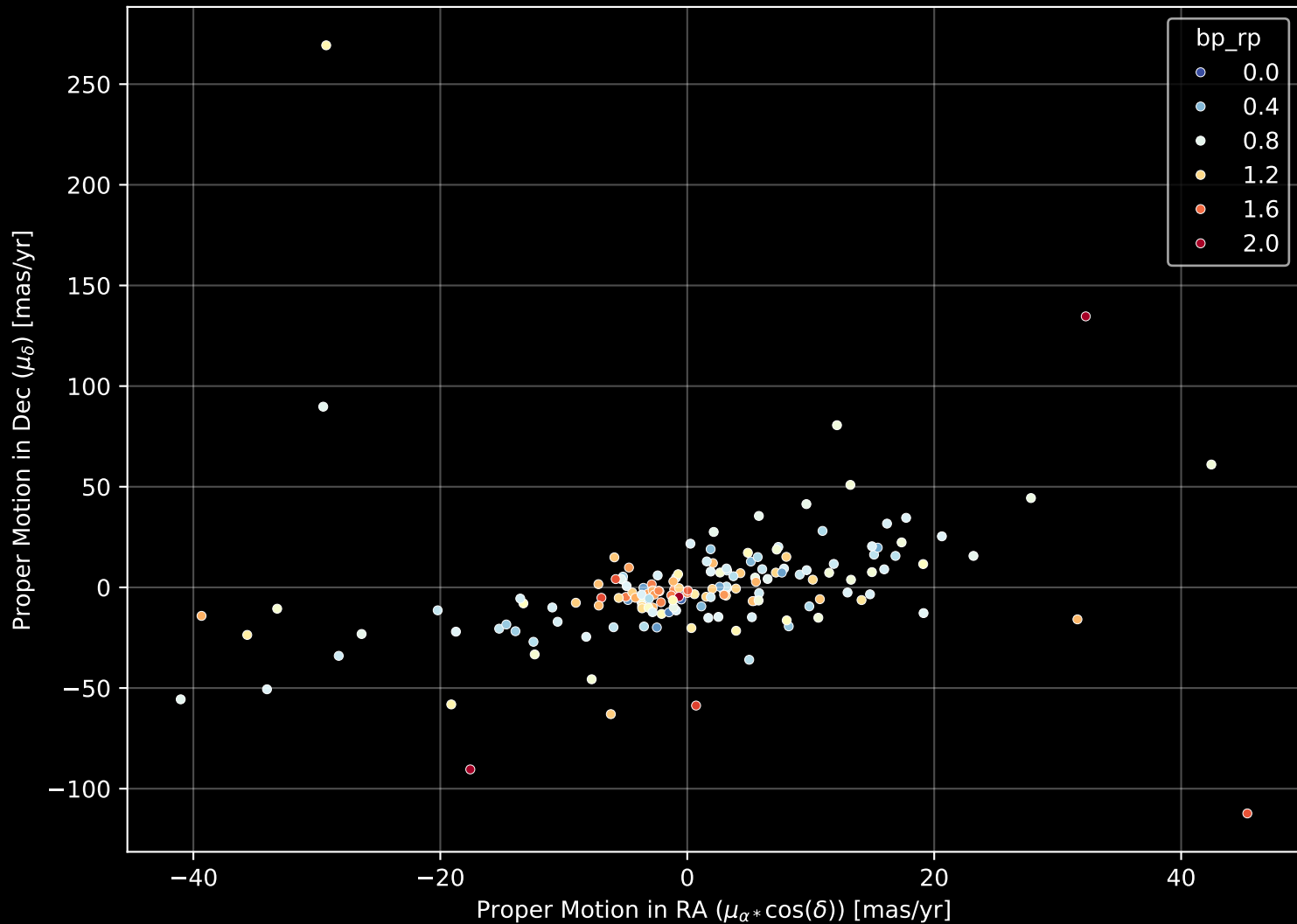
APOGEE DR17 Field: [CVZ_OB02_btx] Proper Motion Diagram (n= 165)
