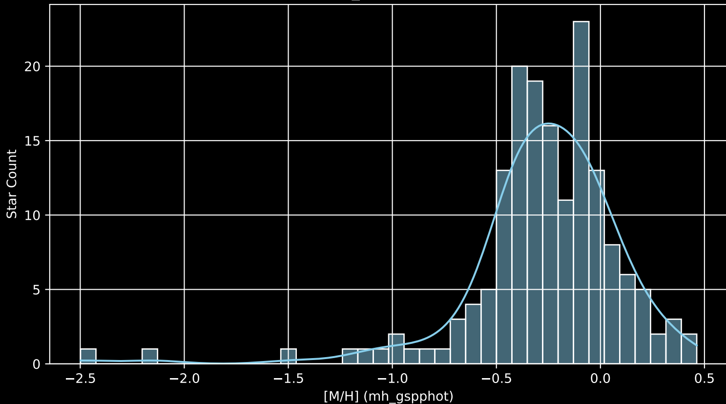
APOGEE DR17 Field: [CVZ_OB02_btx [M/H] (mh_gspphot) (n= 164)
