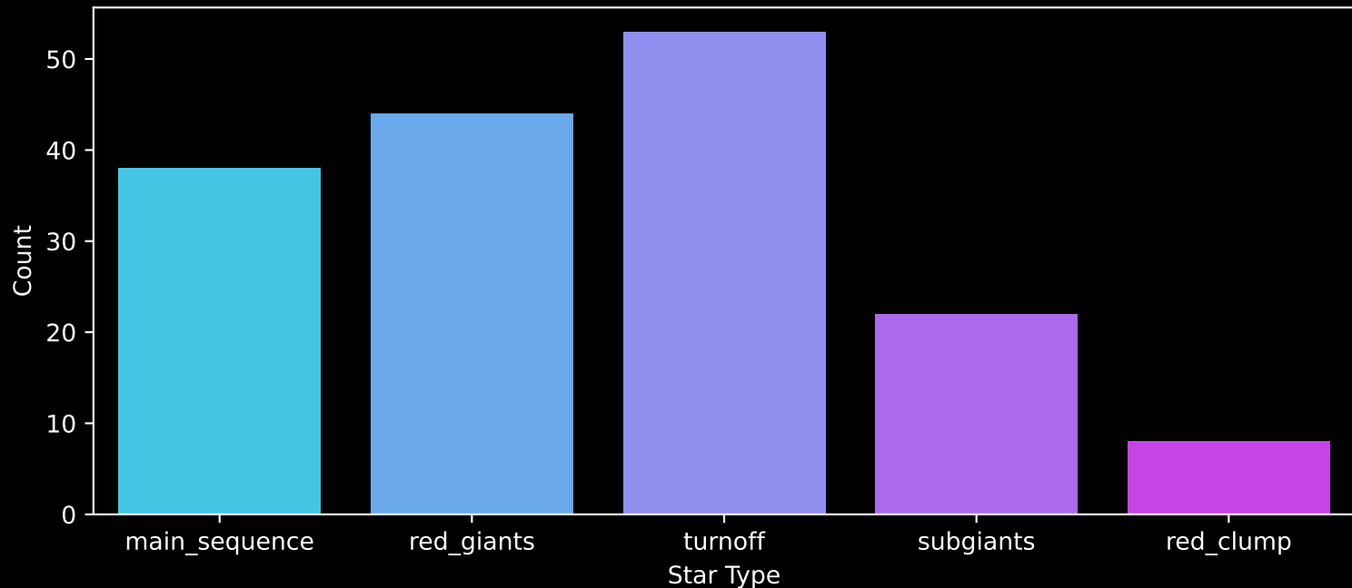
APOGEE DR17 Field: [CVZ_OB02_btx] Count plot of Star Type
