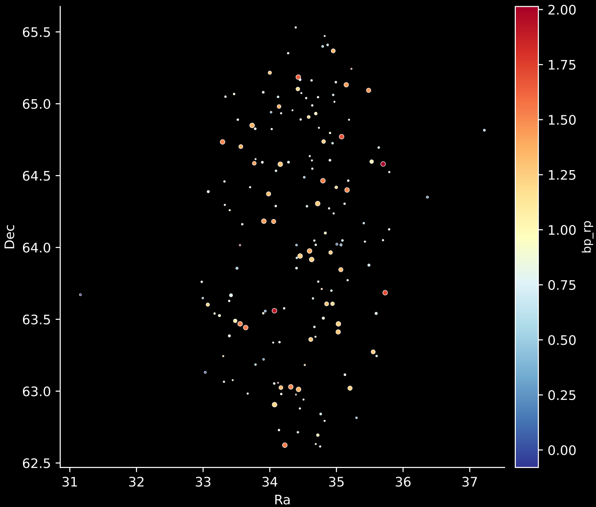
APOGEE DR17 Field: [CVZ_OB02_btx] Stars: 165
