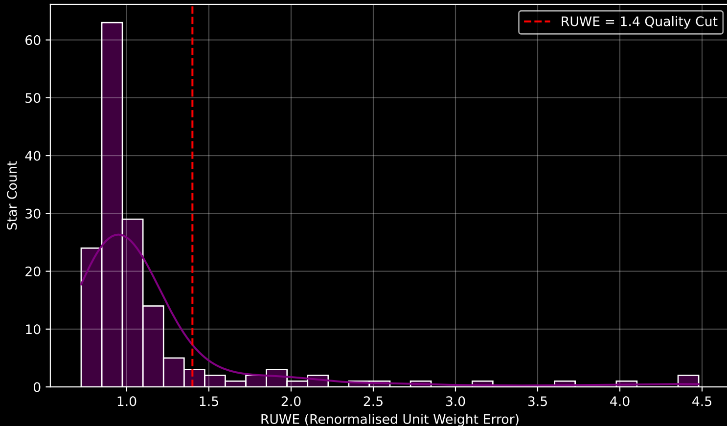
GAPOGEE DR17 Field [CVZ_OB02_btx] RUWE Distribution (n= 157)
